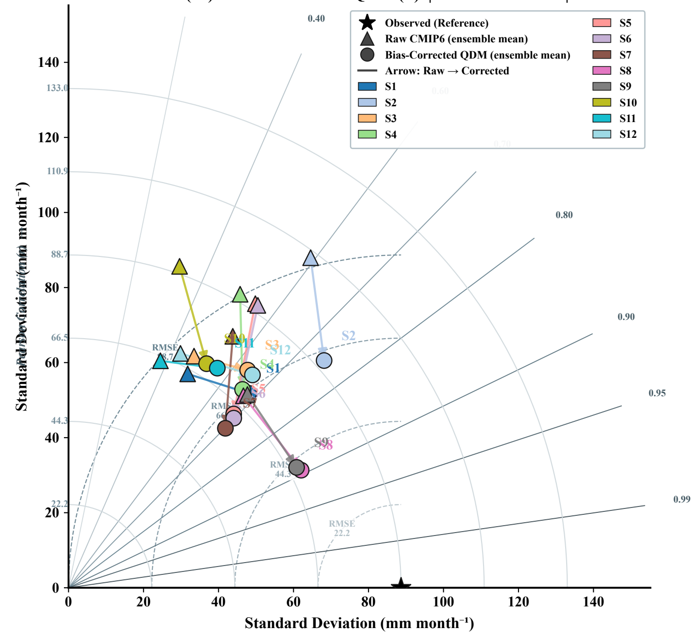
(b) Taylor Diagram — Monthly Scale
