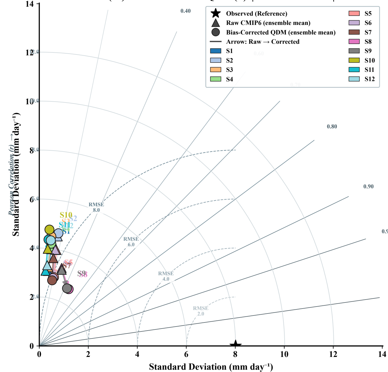
(a) Taylor Diagram — Daily Scale
